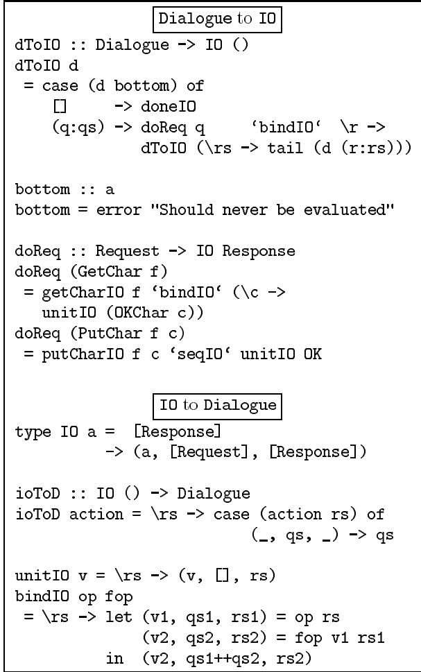
Figure 1: Converting between Dialogue and IO
